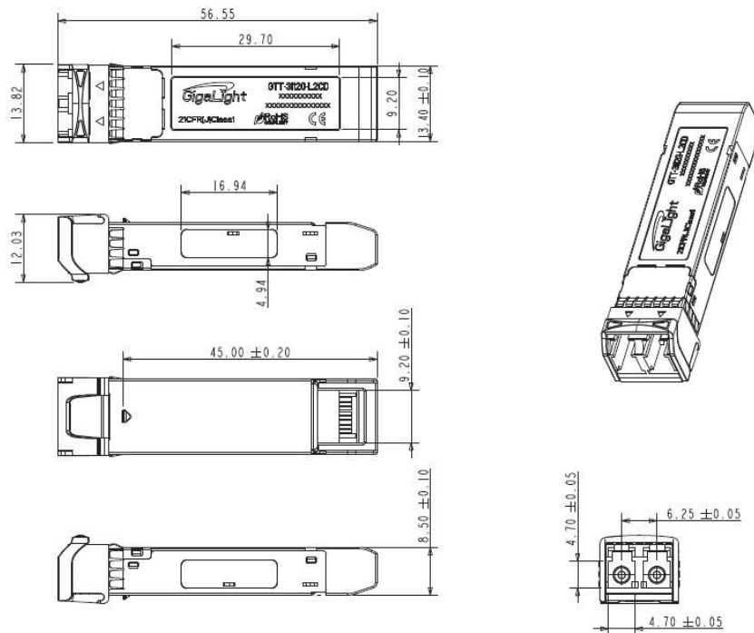
Figure 3. Mechanical Specifications
