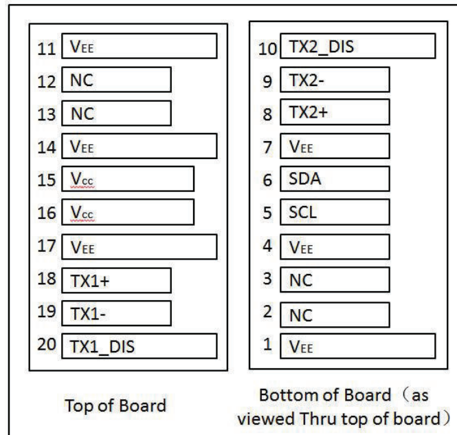
Figure 2. Electrical Pin-out Details
